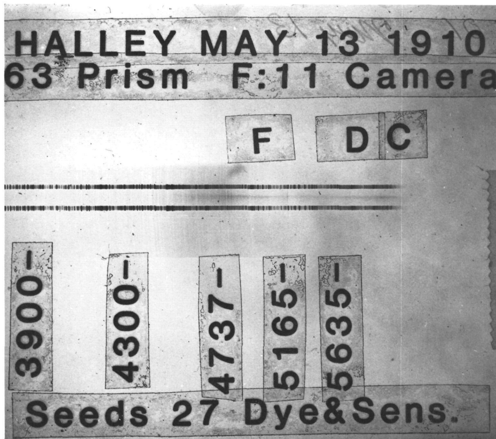
Figure 10. Slit spectrogram of Comet Halley obtained on May 13, 1910.
